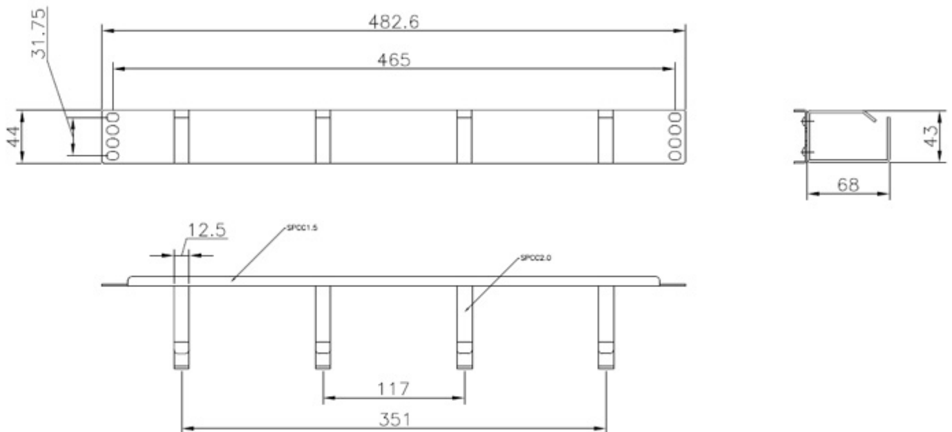
110-582 Excel 1U Cable Management Bar, 4 Vertical Metal Hoops, Black (RAL 9004) - Painted Steel
