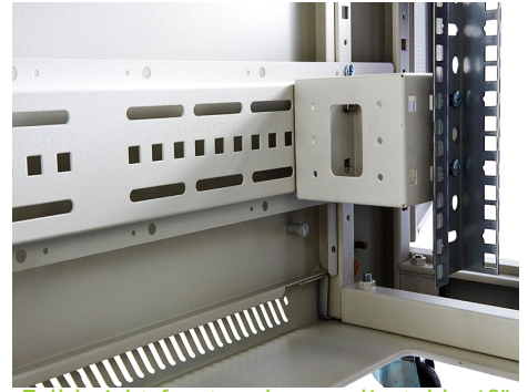
Full height front and rear adjustable 19" profiles
