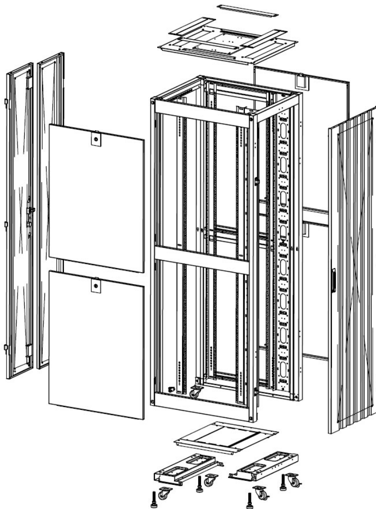
Swing handle 2 point lock fitted to front door
